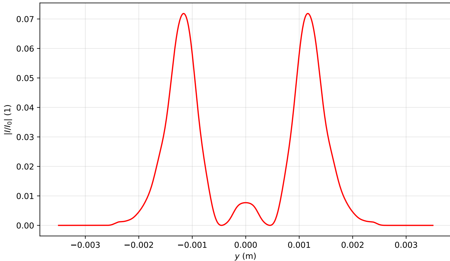
Intensity profile I(x=0, y, z=3.582)/I_0 , P_{in}=7.5P_{cr} , artificial time
